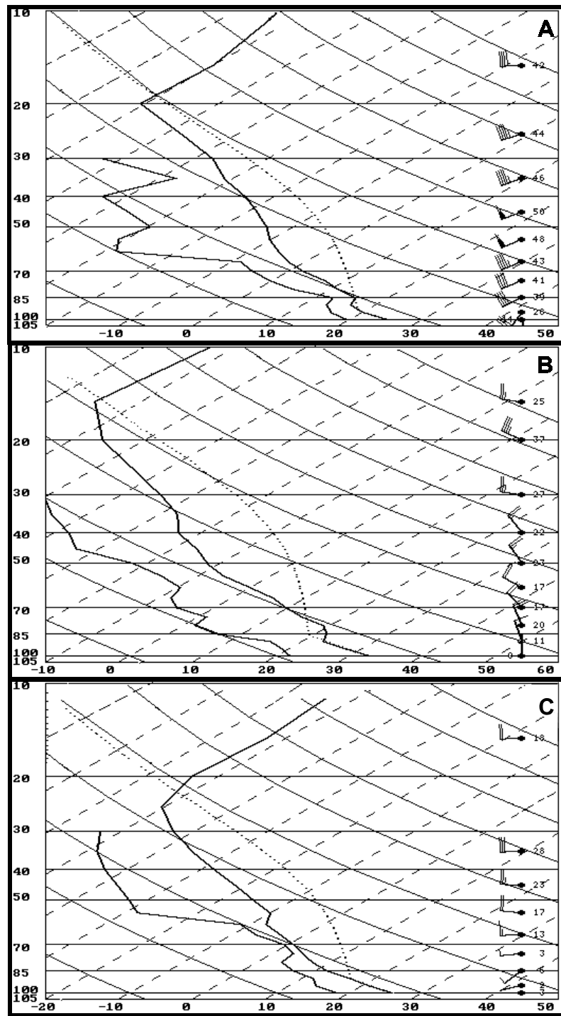
Fig. 3. Soundings for 29 May 1995 (A); 20 June 1995 (B); and 11 July 1995 (C) with the horizontal axis temperature ( ^{\circ}\text{C} ) and vertical axis pressure (mb / 10). Solid lines represent environmental temperature (right) and dewpoint (left). The dotted line indicates the path of a surface-based lifted parcel. Wind barbs (kt) along the right side are plotted using the standard convention.
